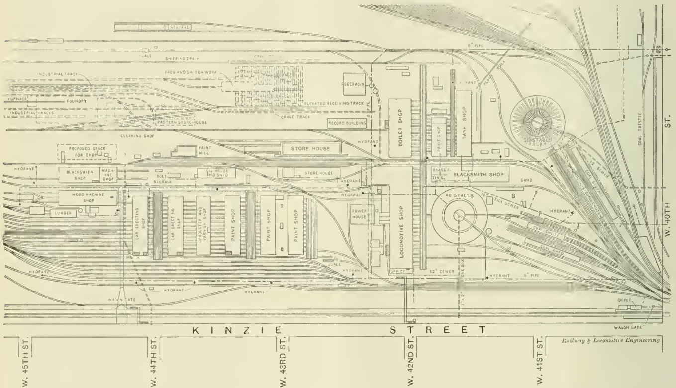
WEST CHICAGO SHOPS OF CHICAGO & NORTHWESTERN.
